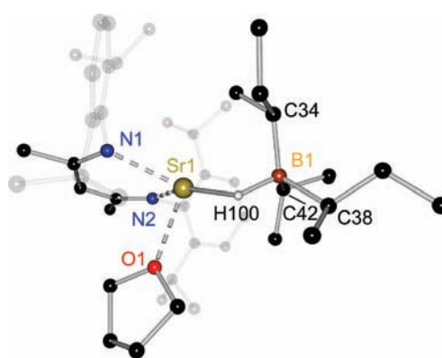
Figure 3. Crystal structure of 4 . The substituents on the nitrogen atoms are depicted transparent, and all hydrogen atoms, except the hydrogen atom involved in bonding to \text{Sr}^{2+} , have been omitted for clarity. For selected bond distances (Å) and angles (°) see Table 1.
